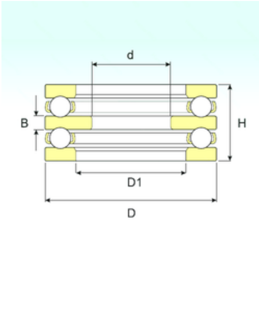
52230 M Bearing 2D drawings and 3D CAD models
